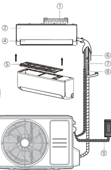
Outdoor power supply models
